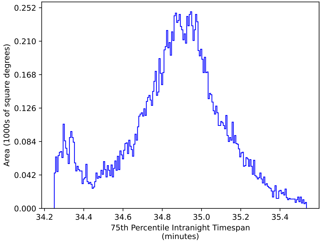
roll_uniform_early_half_mjdp253_v3.4_10yrs WFD: 75th Percentile Intranight Timespan
