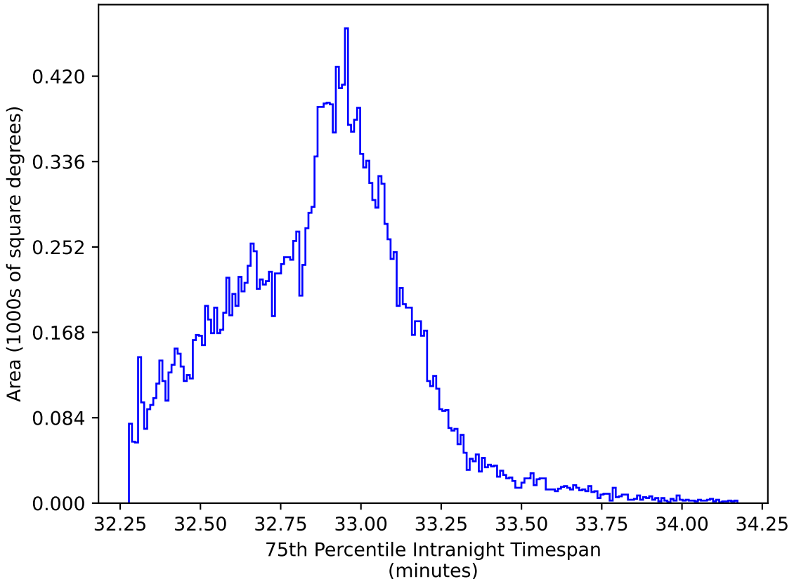
roll_uniform_early_half_mjdp253_v3.4_10yrs All sky y band: 75th Percentile Intranight Timespan
