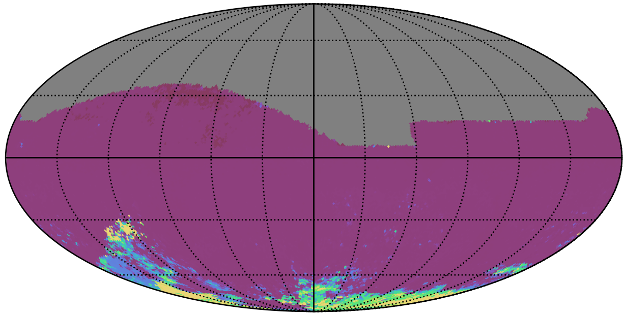
roll_uniform_early_half_mjdp253_v3.4_10yrs All sky ri bands: 75th Percentile Intranight Timespan
