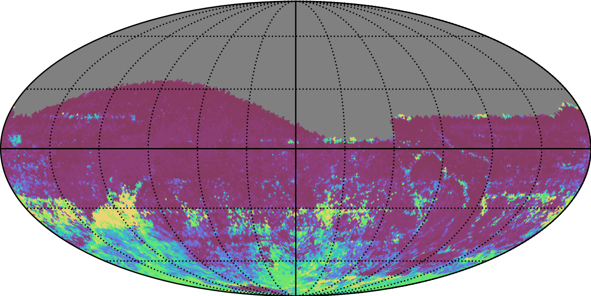
roll_uniform_early_half_mjdp253_v3.4_10yrs All sky r band: 75th Percentile Intranight Timespan
