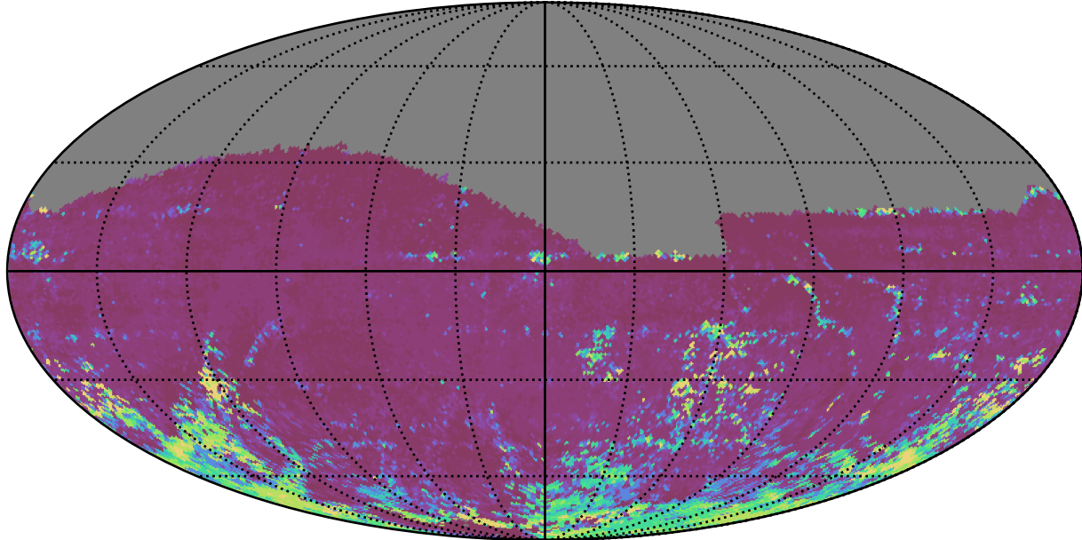
roll_uniform_early_half_mjdp253_v3.4_10yrs All sky i band: 75th Percentile Intranight Timespan
