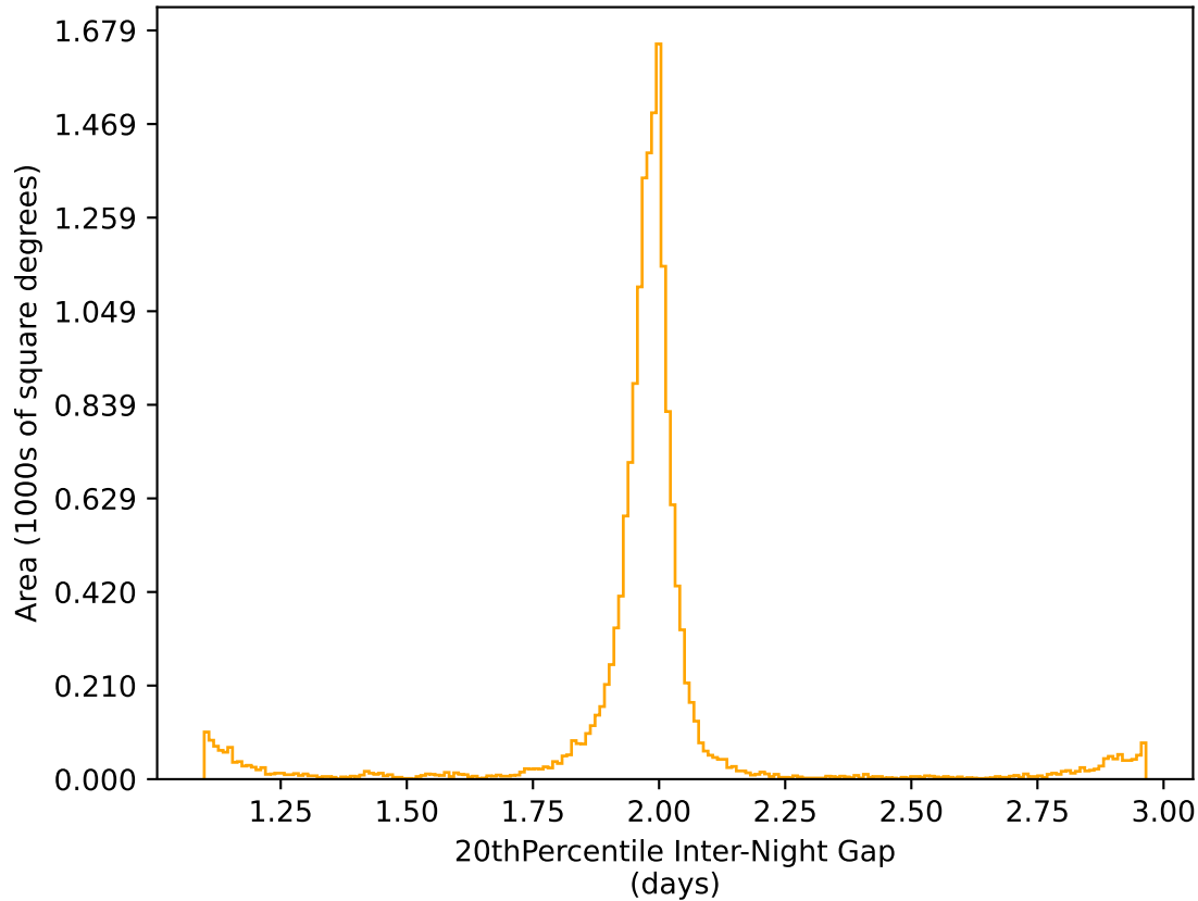
roll_uniform_early_half_mjdp253_v3.4_10yrs WFD r band: 20thPercentile Inter-Night Gap
