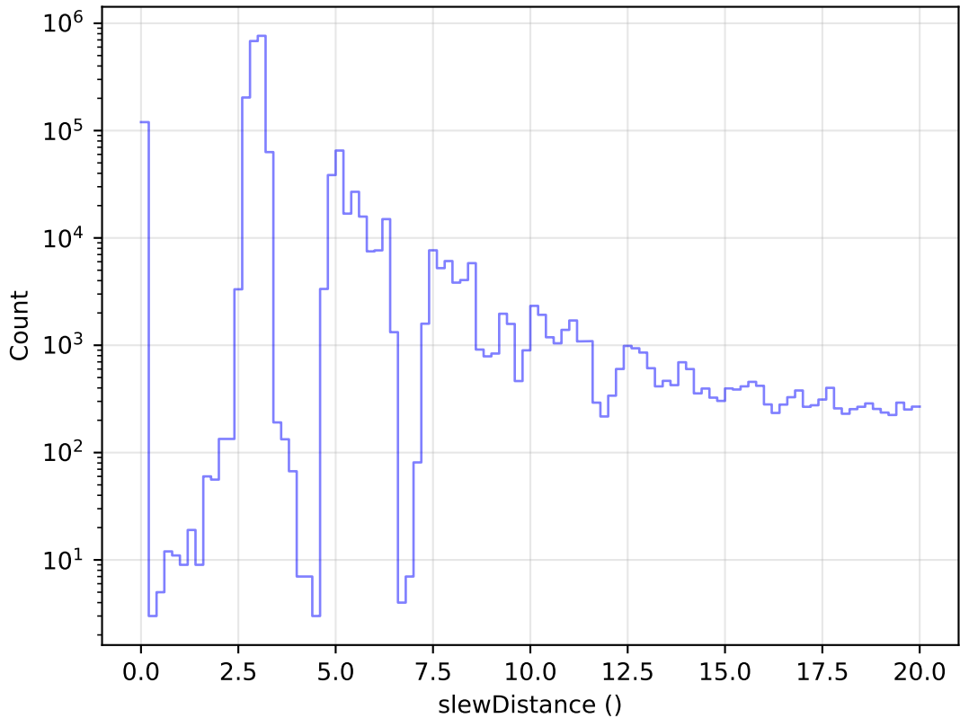
roll_uniform_early_half_mjdp253_v3.4_10yrs All visits: Zoom Slew Distance Histogram
