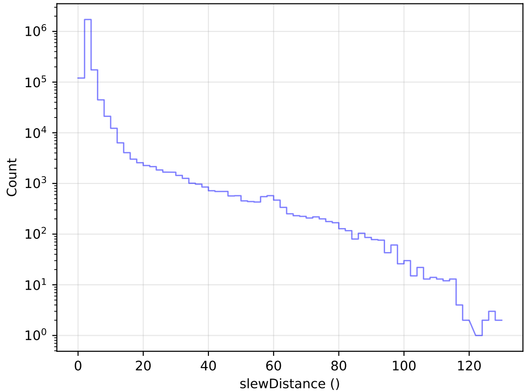
roll_uniform_early_half_mjdp253_v3.4_10yrs All visits: Slew Distance Histogram
