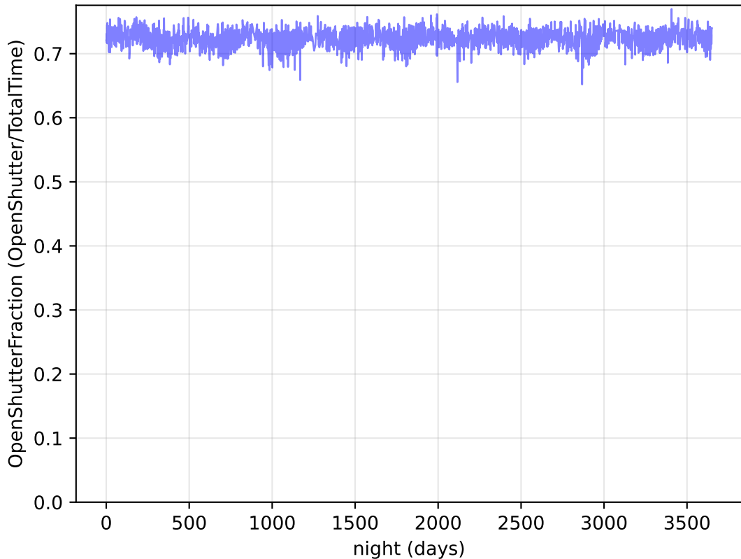
roll_uniform_early_half_mjdp253_v3.4_10yrs : OpenShutterFraction
