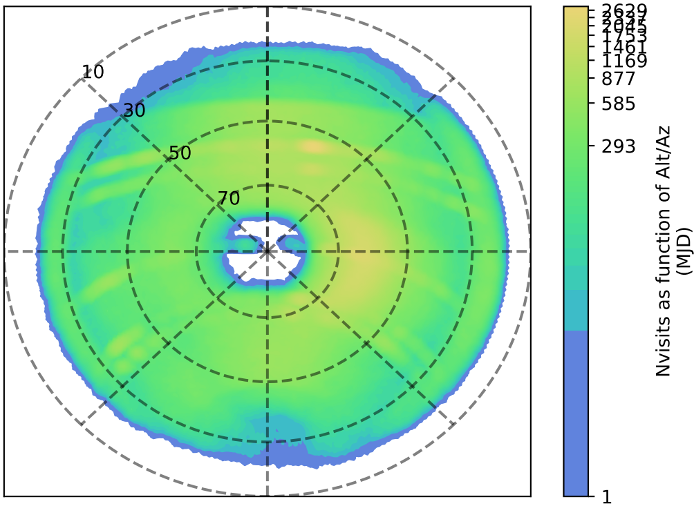
roll_uniform_early_half_mjdp253_v3.4_10yrs z: Nvisits as function of Alt/Az
