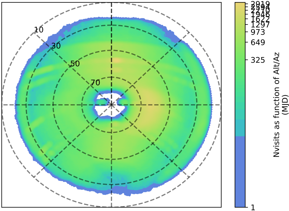
roll_uniform_early_half_mjdp253_v3.4_10yrs i: Nvisits as function of Alt/Az
