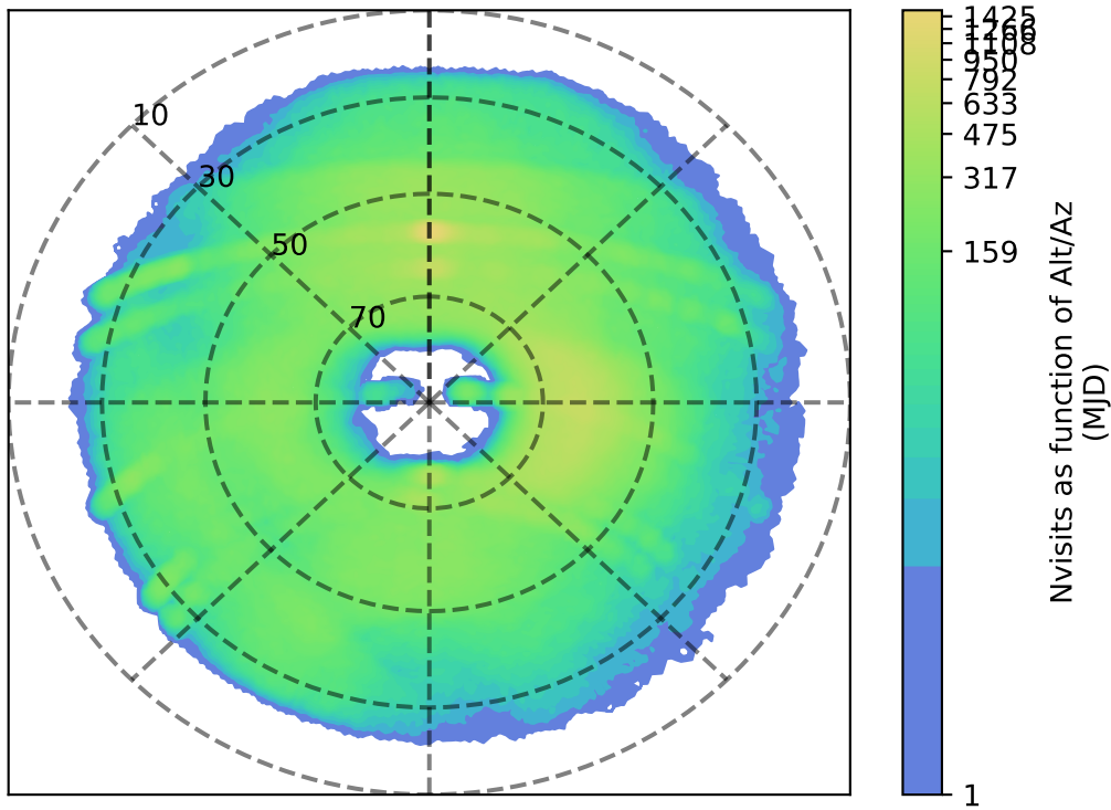
roll_uniform_early_half_mjdp253_v3.4_10yrs g: Nvisits as function of Alt/Az
