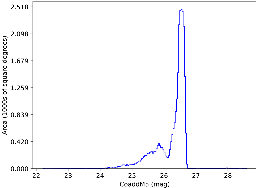
roll_uniform_early_half_mjdp253_v3.4_10yrs i: CoaddM5
