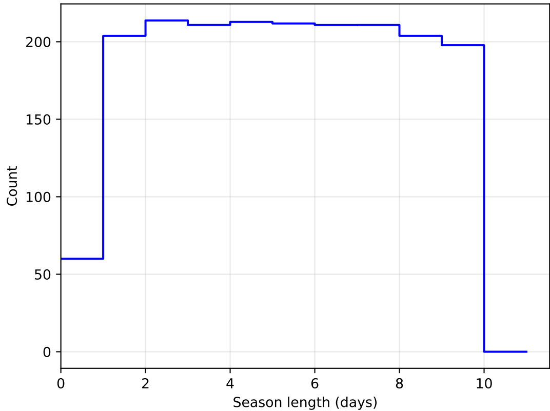
roll_uniform_early_half_mjdp253_v3.4_10yrs DD:EDFS all bands: SeasonLength
