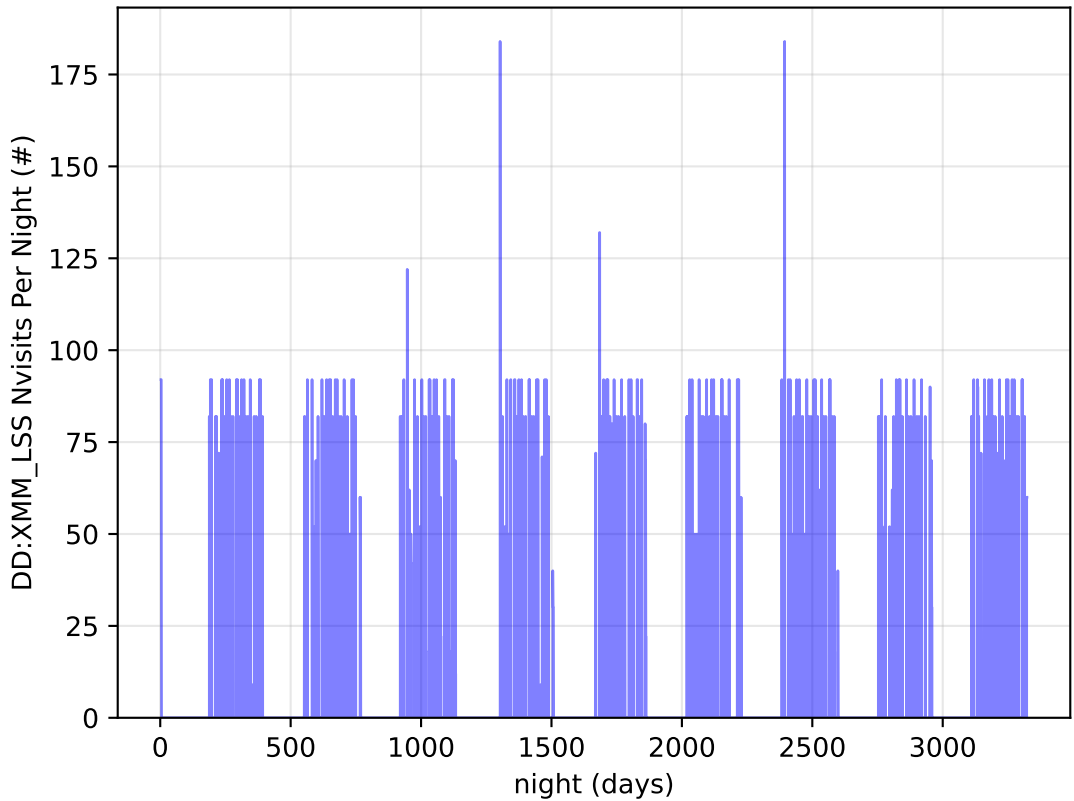
roll_uniform_early_half_mjdp253_v3.4_10yrs all bands: DD:XMM_LSS Nvisits Per Night
