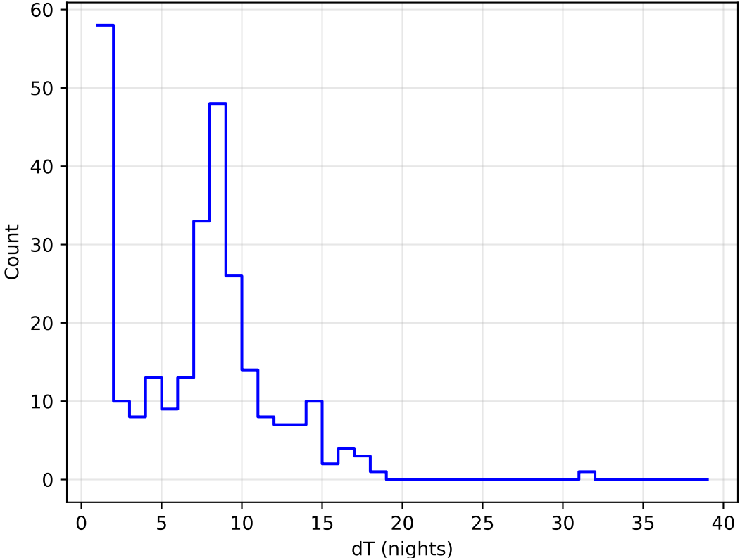
roll_uniform_early_half_mjdp253_v3.4_10yrs all bands: DD:XMM_LSS Delta Nights Histogram
