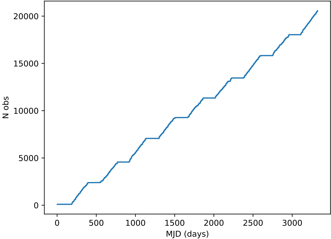
roll_uniform_early_half_mjdp253_v3.4_10yrs all bands: DD:XMM_LSS Cumulative NVisits
