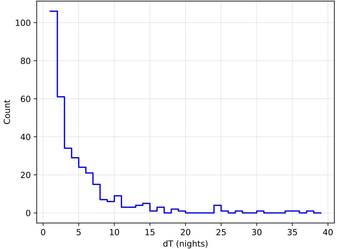
roll_uniform_early_half_mjdp253_v3.4_10yrs all bands: DD:WFD Delta Nights Histogram
