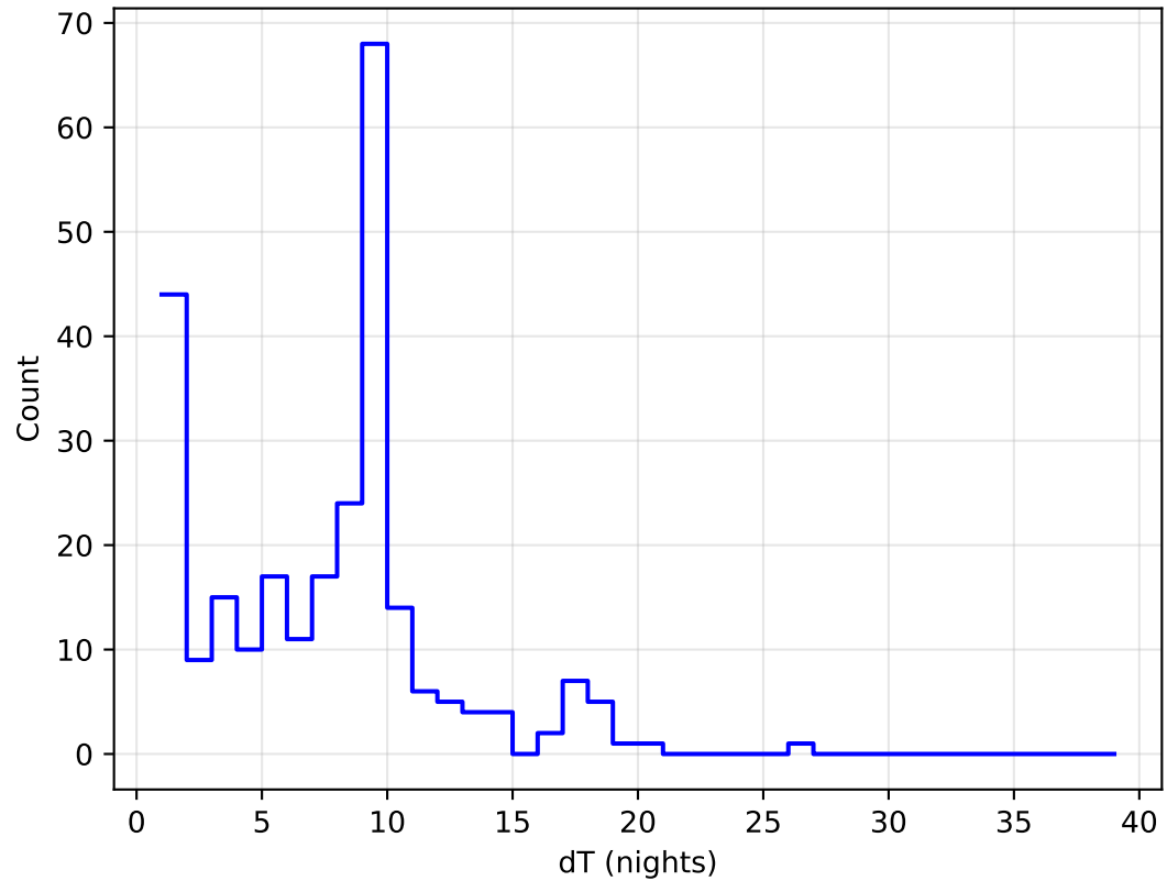
roll_uniform_early_half_mjdp253_v3.4_10yrs all bands: DD:ELAISS1 Delta Nights Histogram
