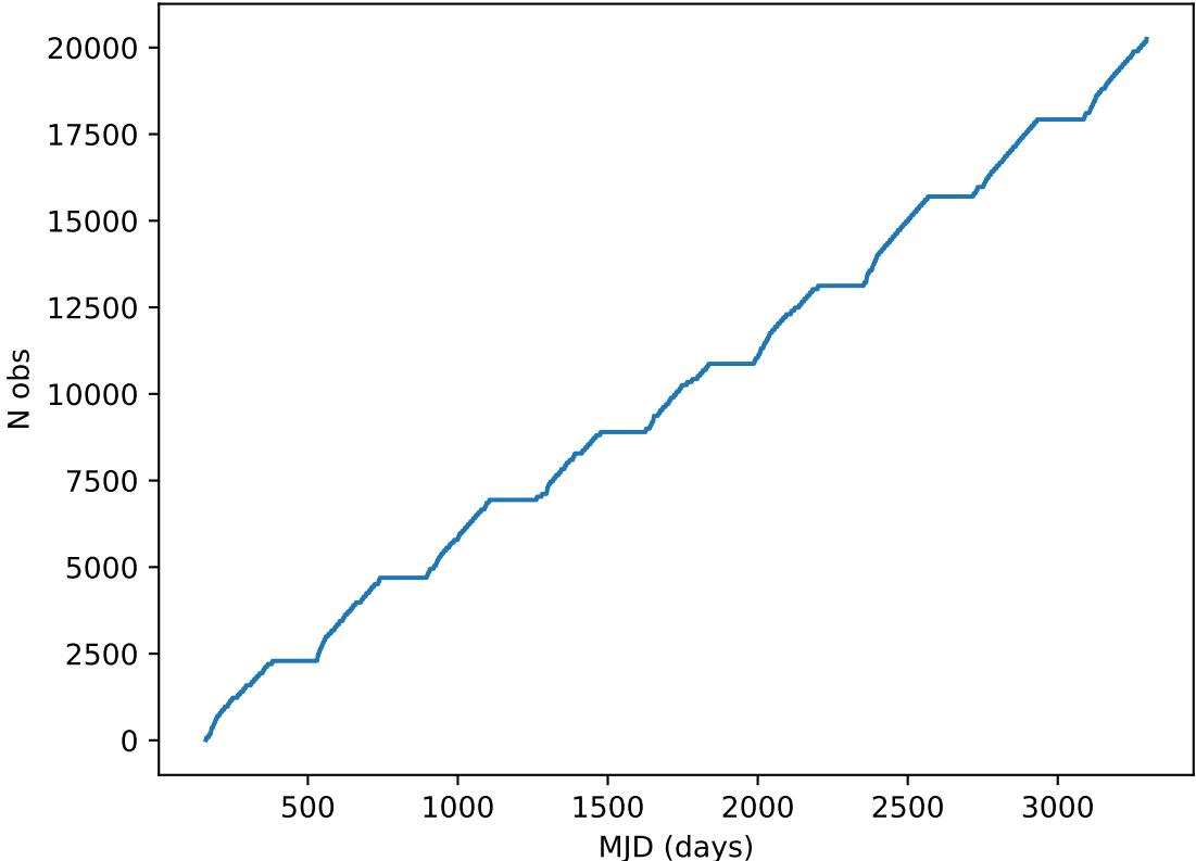
roll_uniform_early_half_mjdp253_v3.4_10yrs all bands: DD:ELAISS1 Cumulative NVisits
