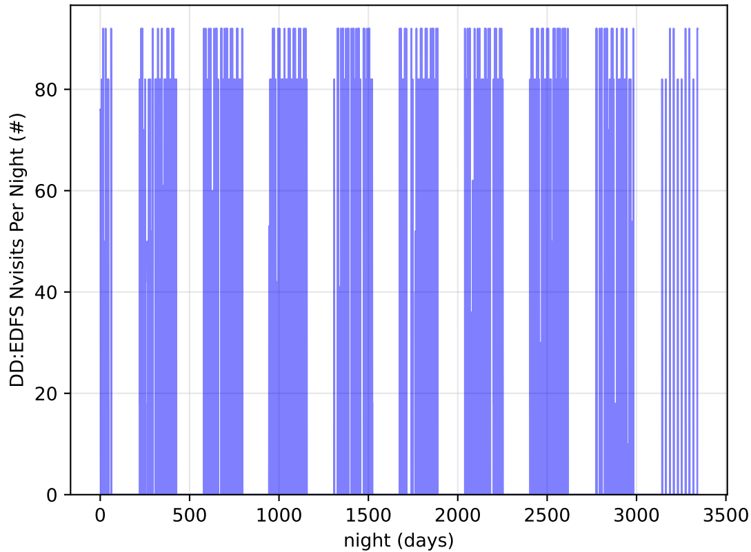
roll_uniform_early_half_mjdp253_v3.4_10yrs all bands: DD:EDFS Nvisits Per Night
