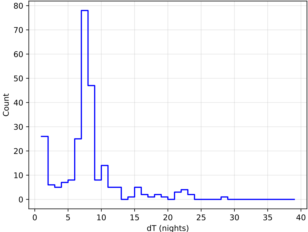
roll_uniform_early_half_mjdp253_v3.4_10yrs all bands: DD:EDFS Delta Nights Histogram
