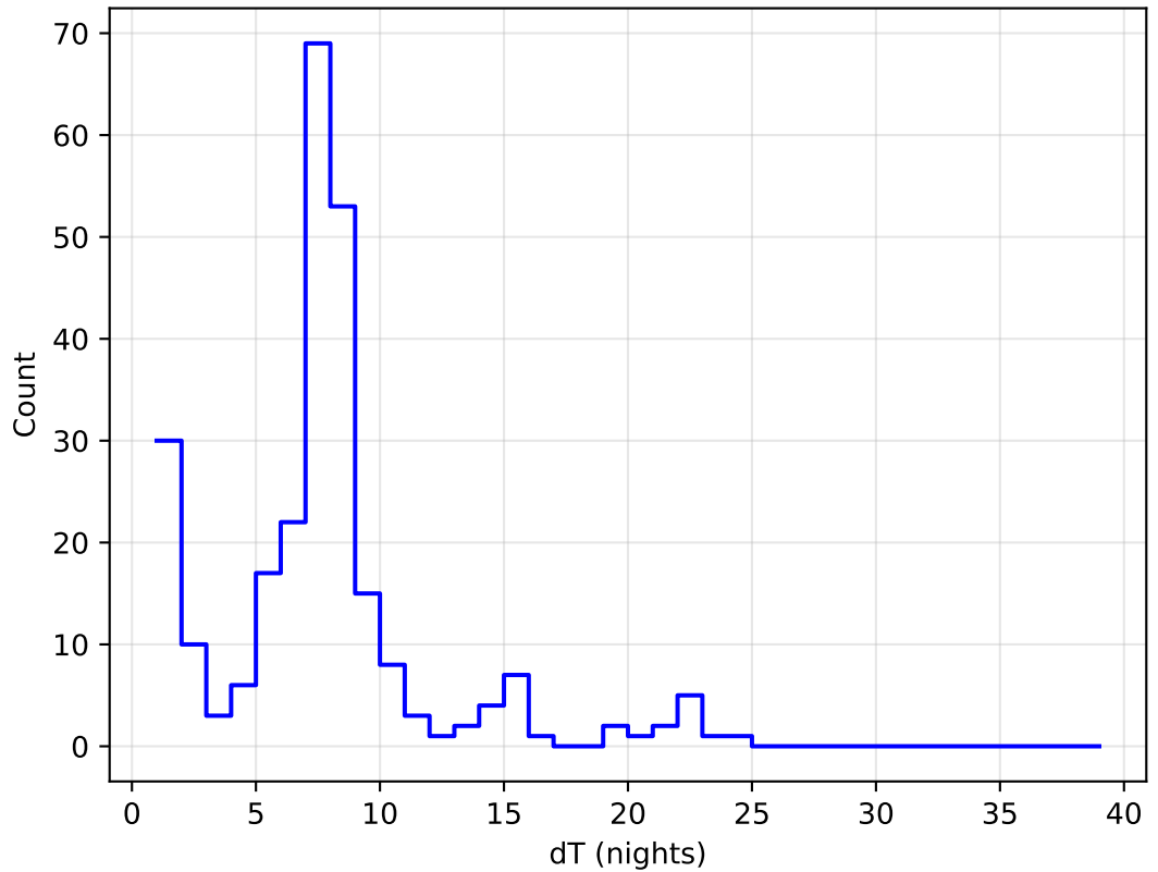
roll_uniform_early_half_mjdp253_v3.4_10yrs all bands: DD:ECDFS Delta Nights Histogram
