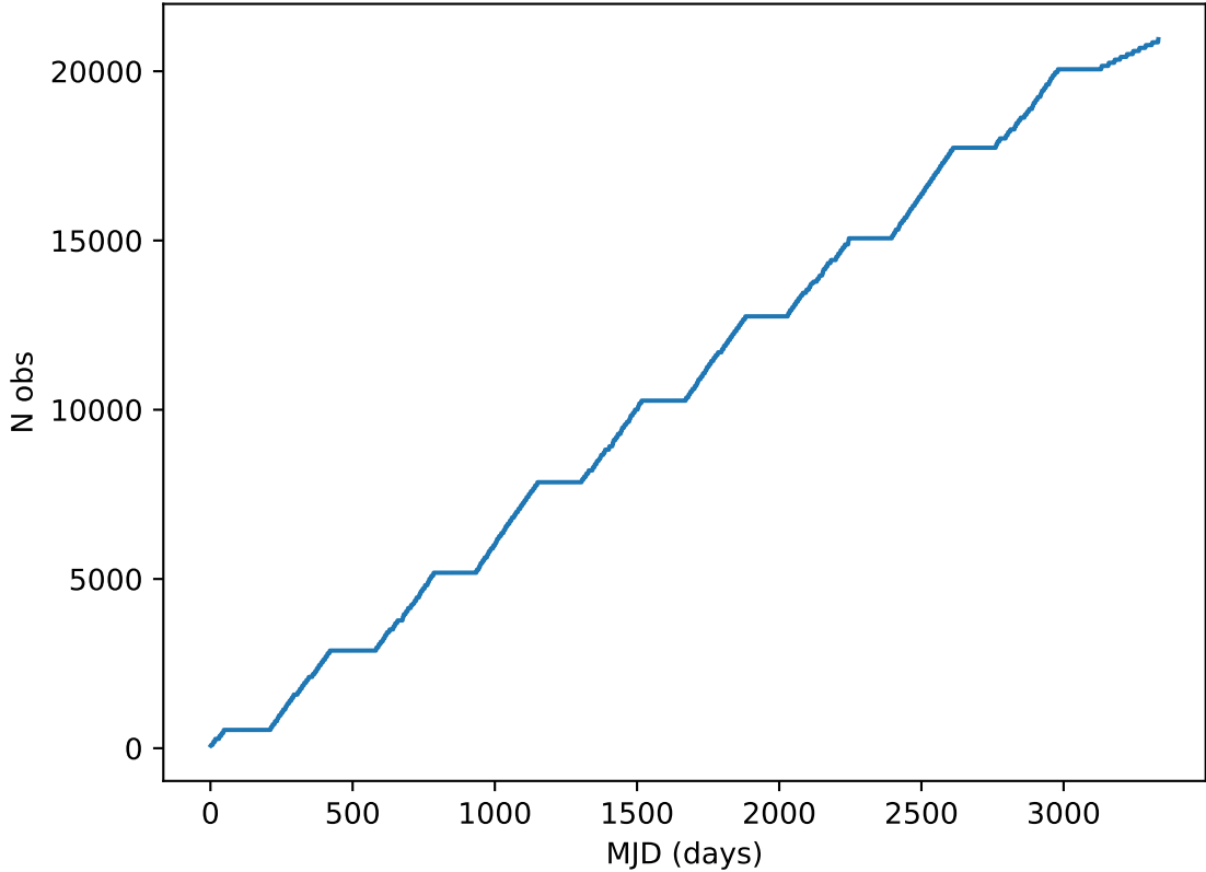
roll_uniform_early_half_mjdp253_v3.4_10yrs all bands: DD:ECDFS Cumulative NVisits
