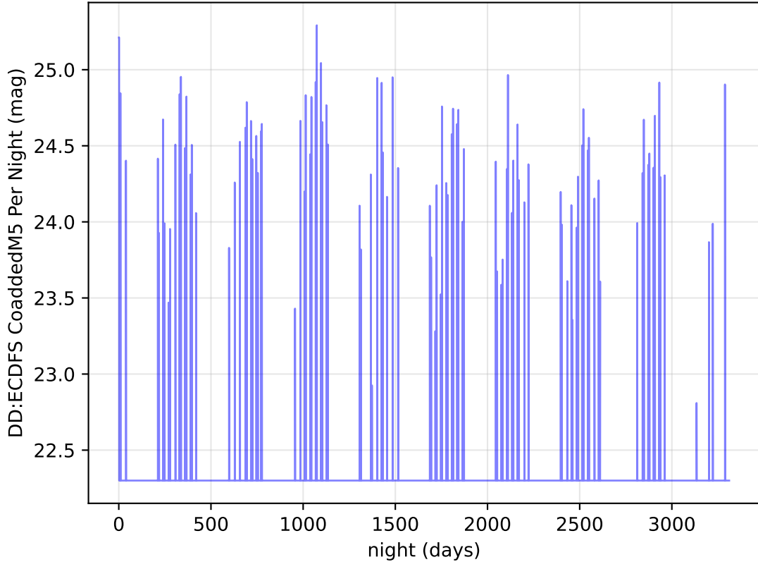
roll_uniform_early_half_mjdp253_v3.4_10yrs u band: DD:ECDFS CoaddedM5 Per Night
