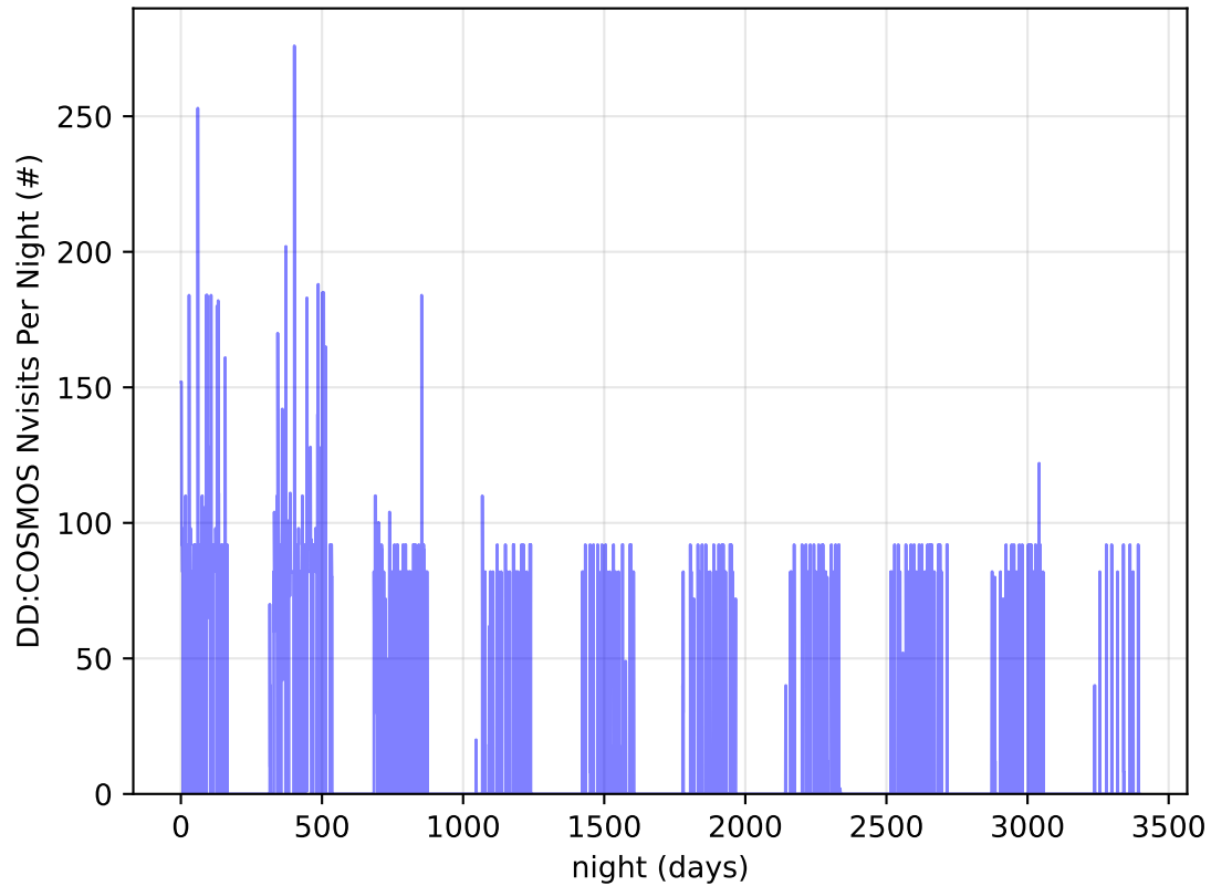
roll_uniform_early_half_mjdp253_v3.4_10yrs all bands: DD: COSMOS Nvisits Per Night
