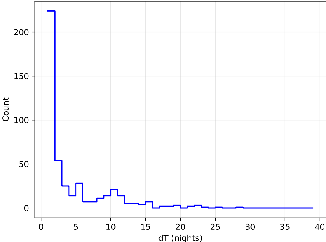
roll_uniform_early_half_mjdp253_v3.4_10yrs all bands: DD:COSMOS Delta Nights Histogram
