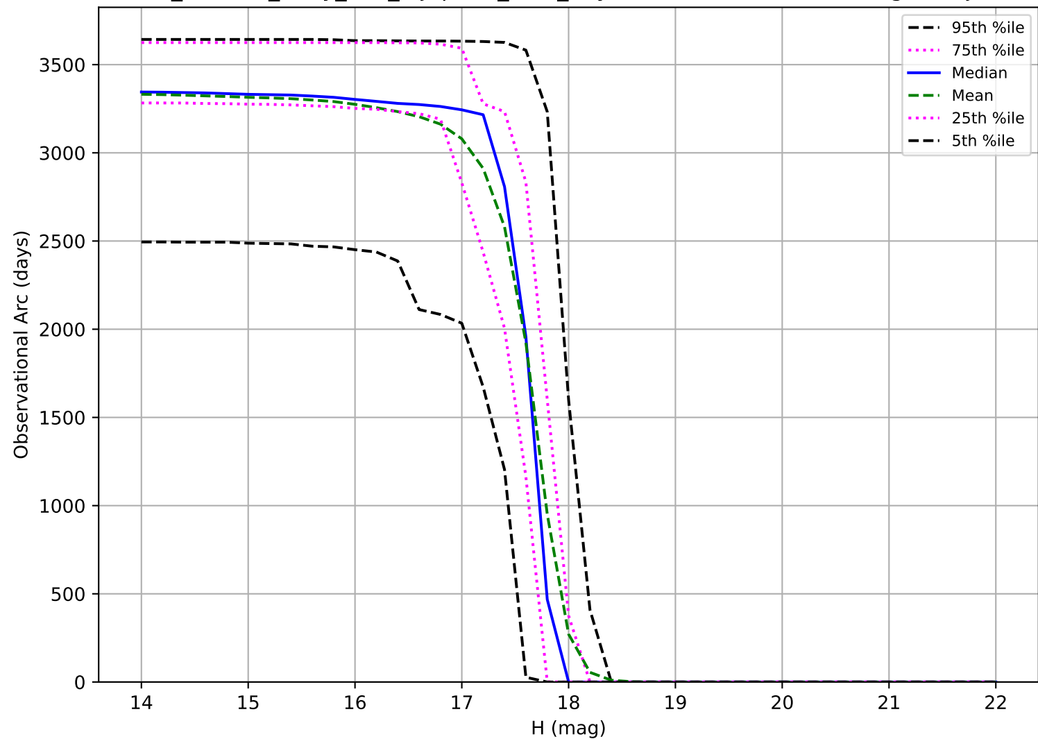
roll_uniform_early_half_mjdp180_v3.4_10yrs: Observational Arc Length Trojan
