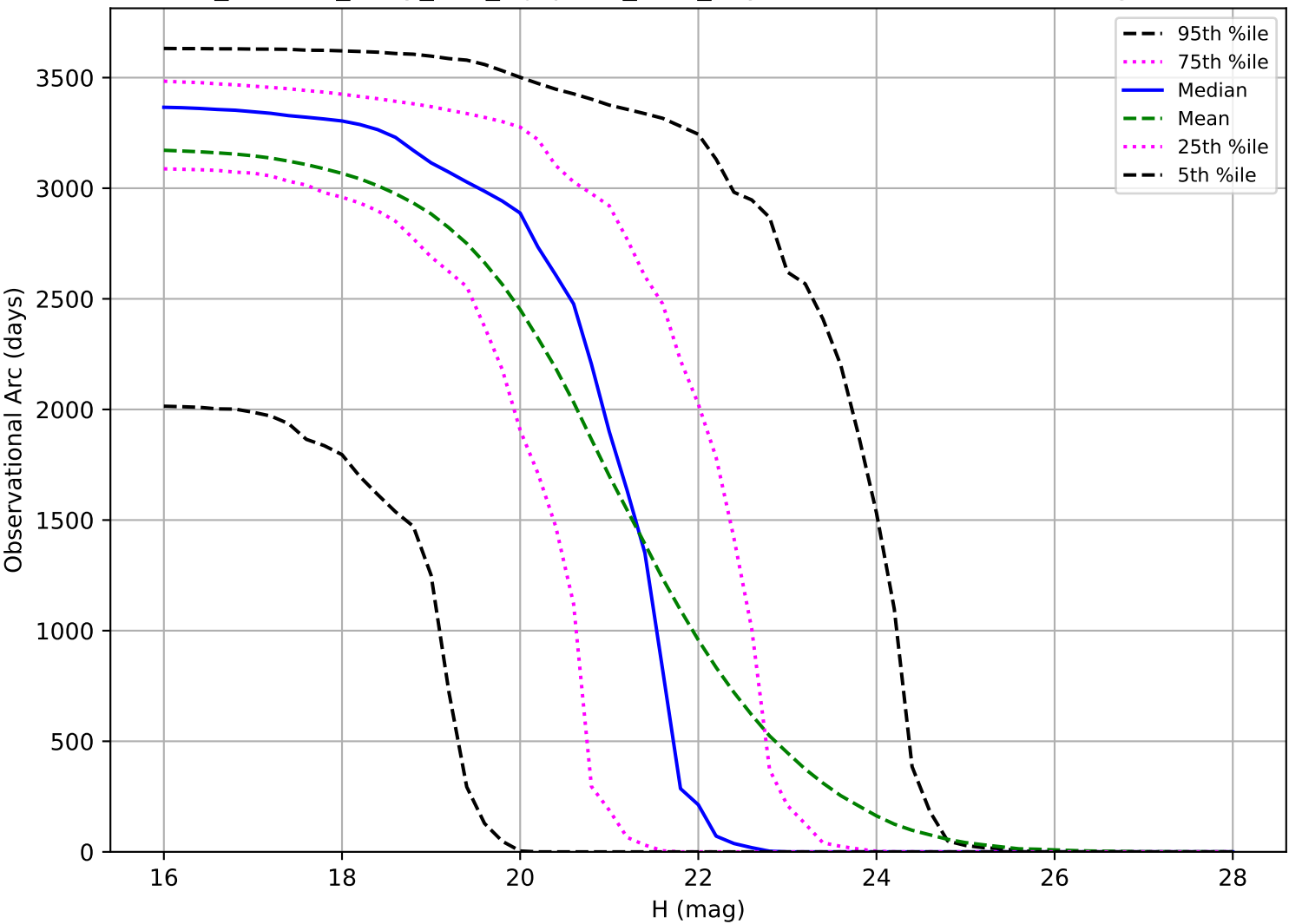
roll_uniform_early_half_mjdp180_v3.4_10yrs: Observational Arc Length PHA
