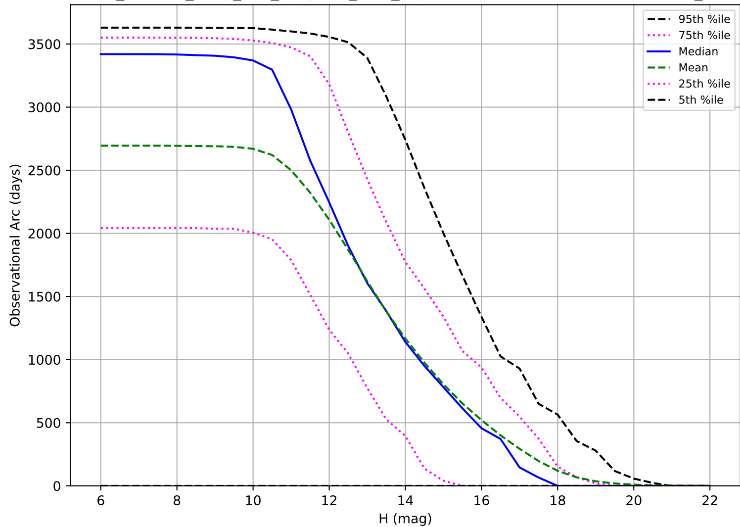
roll_uniform_early_half_mjdp180_v3.4_10yrs: Observational Arc Length OCC_r5
