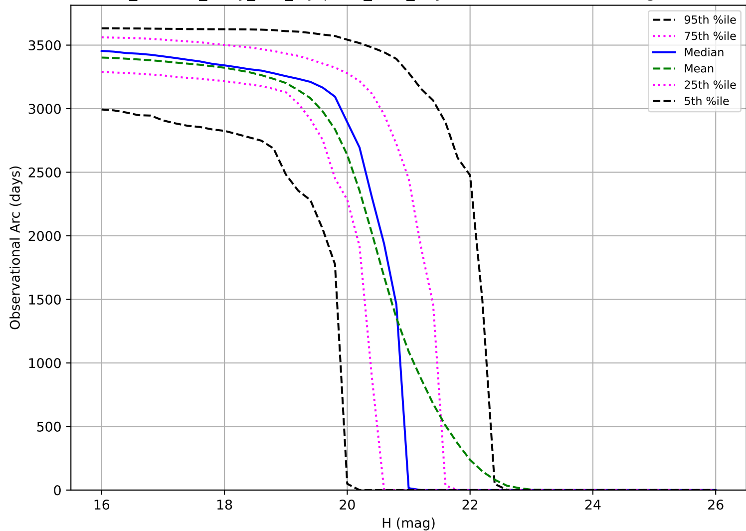
roll_uniform_early_half_mjdp180_v3.4_10yrs: Observational Arc Length MBA
