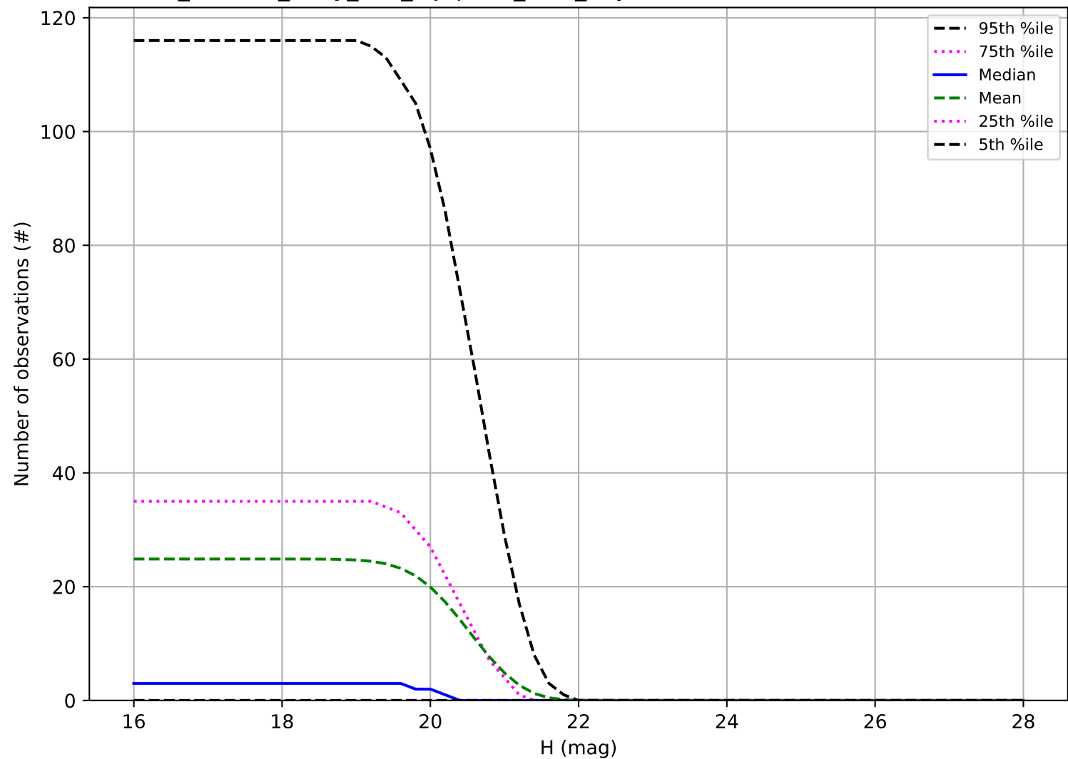
roll_uniform_early_half_mjdp180_v3.4_10yrs: Number of observations Vatira
