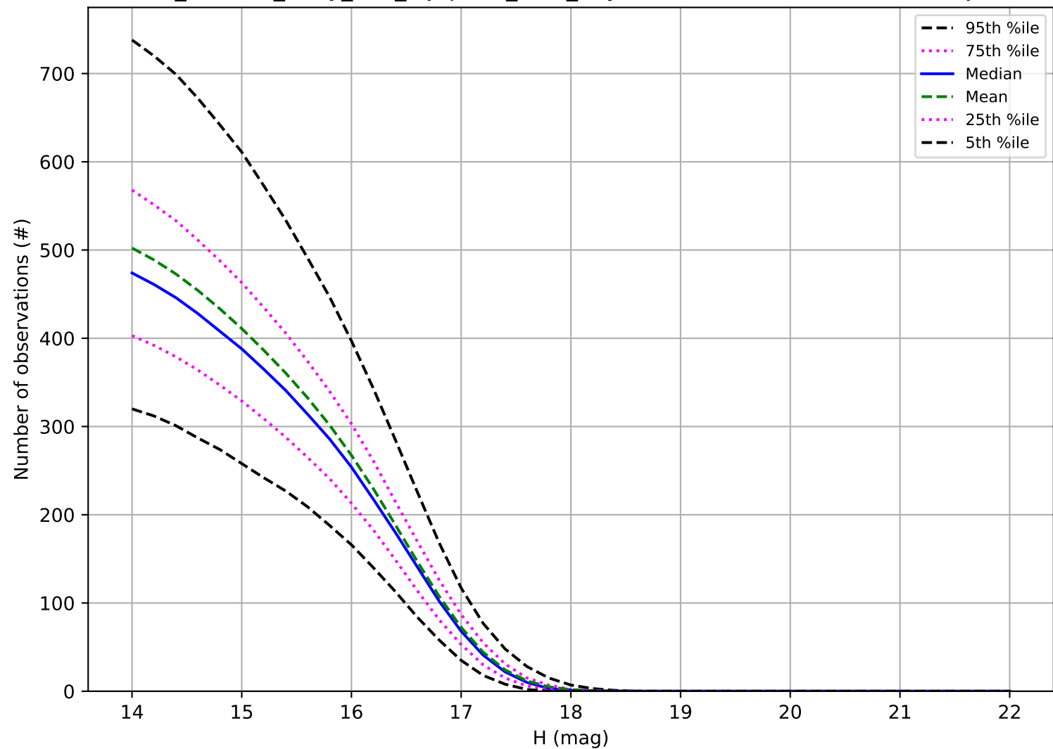
roll_uniform_early_half_mjdp180_v3.4_10yrs: Number of observations Trojan
