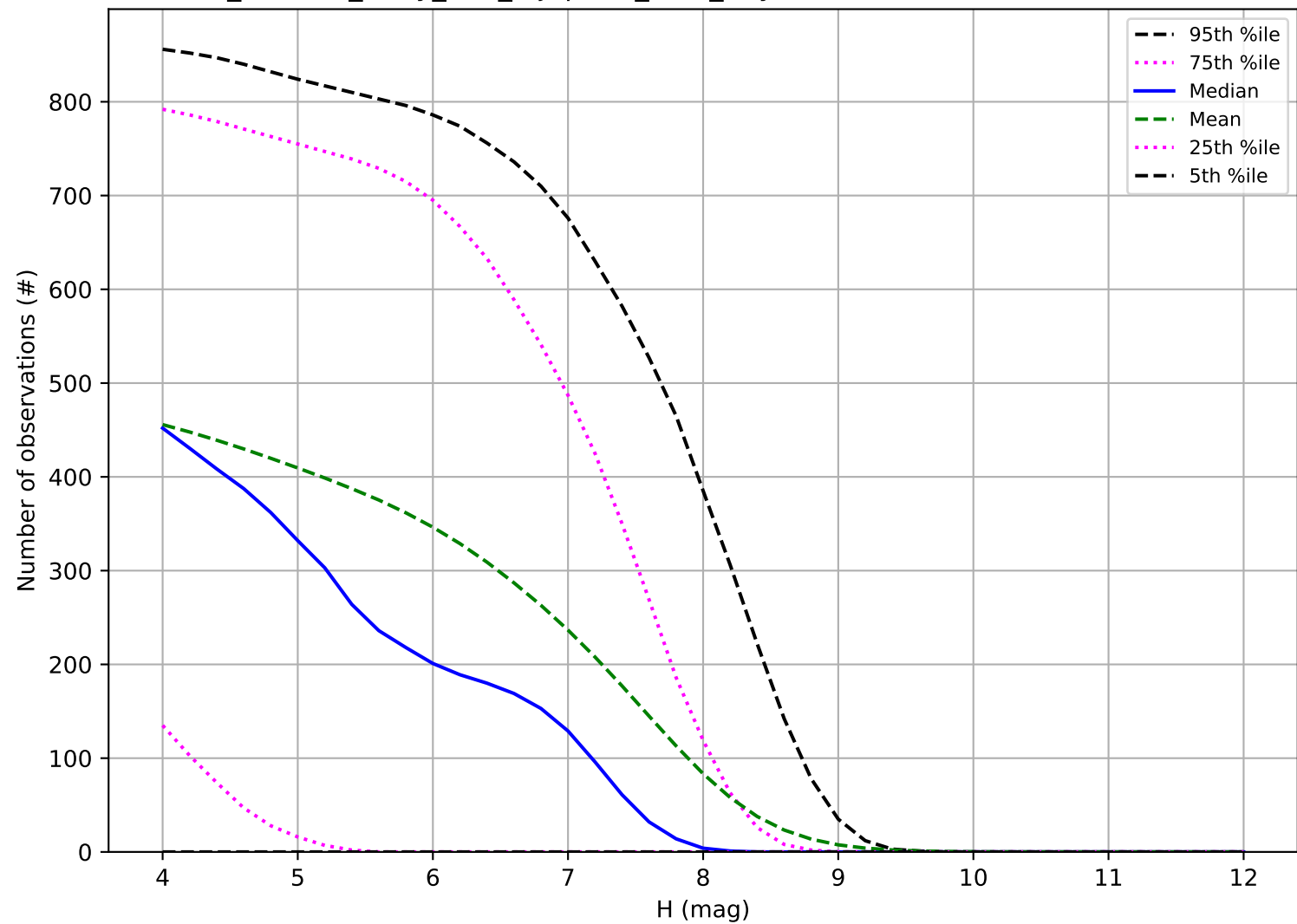
roll_uniform_early_half_mjdp180_v3.4_10yrs: Number of observations TNO
