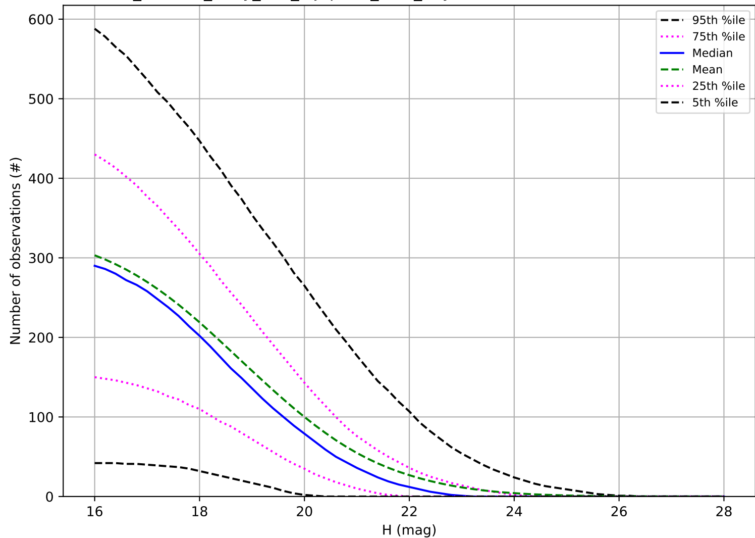
roll_uniform_early_half_mjdp180_v3.4_10yrs: Number of observations PHA
