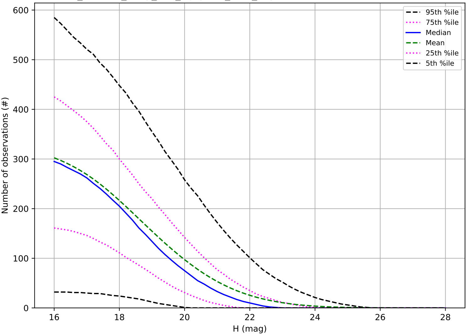
roll_uniform_early_half_mjdp180_v3.4_10yrs: Number of observations NEO
