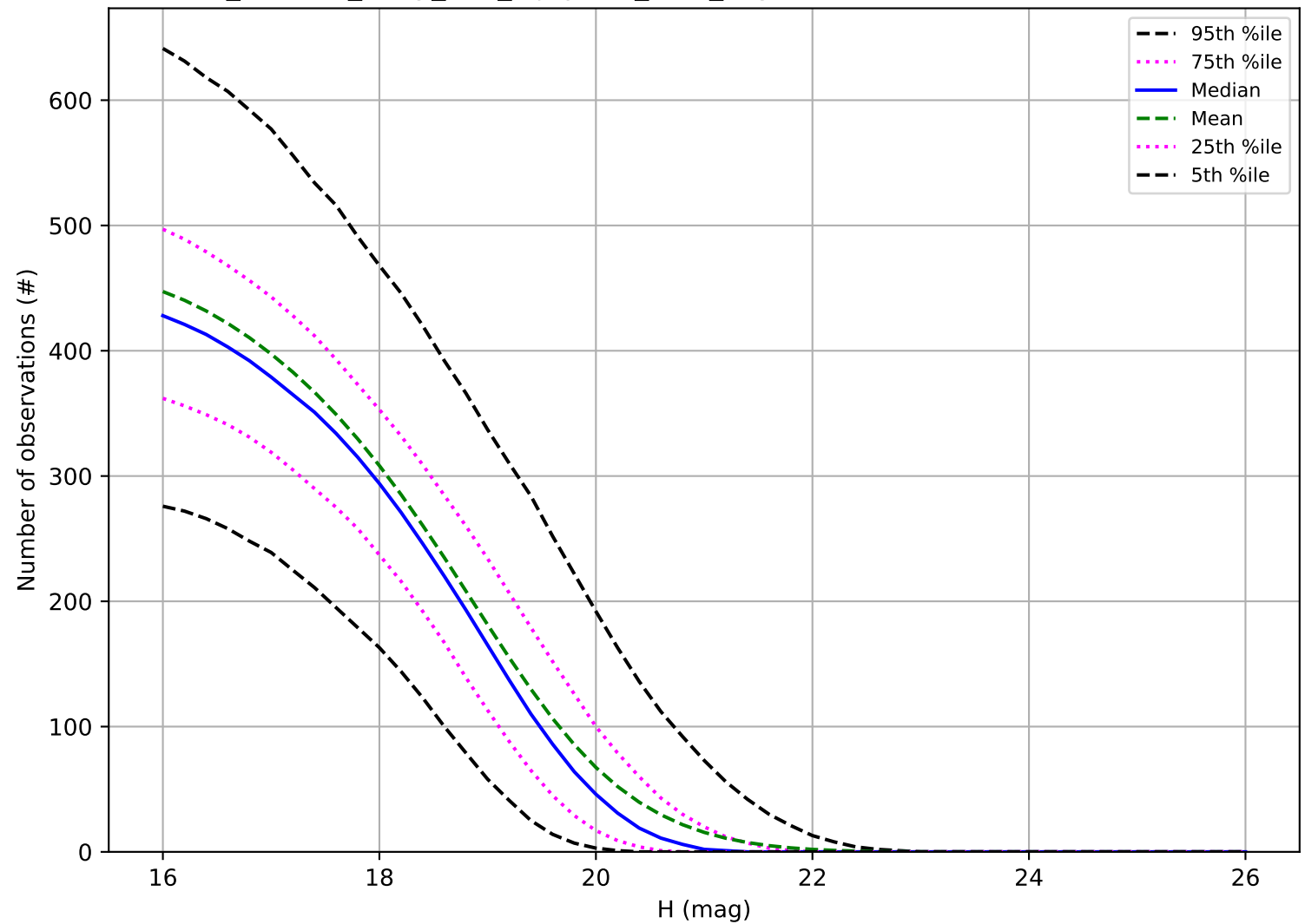
roll_uniform_early_half_mjdp180_v3.4_10yrs: Number of observations MBA
