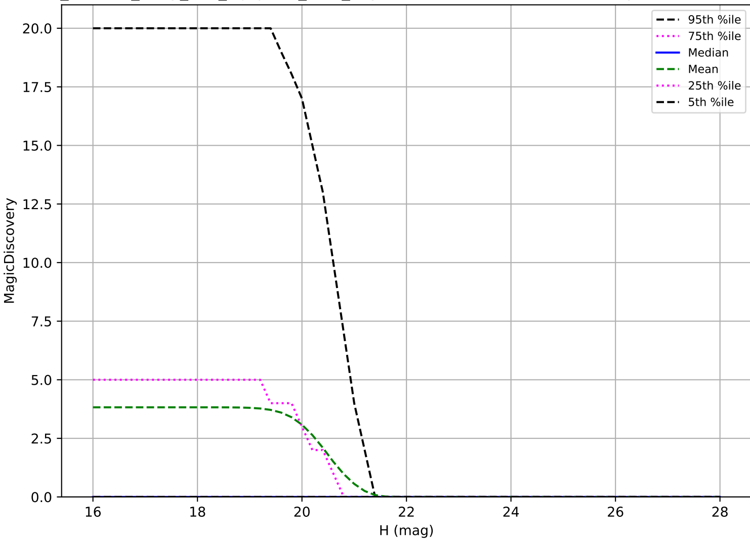
roll_uniform_early_half_mjdp180_v3.4_10yrs: Vatira 6 detections in 60 nights detection loss
