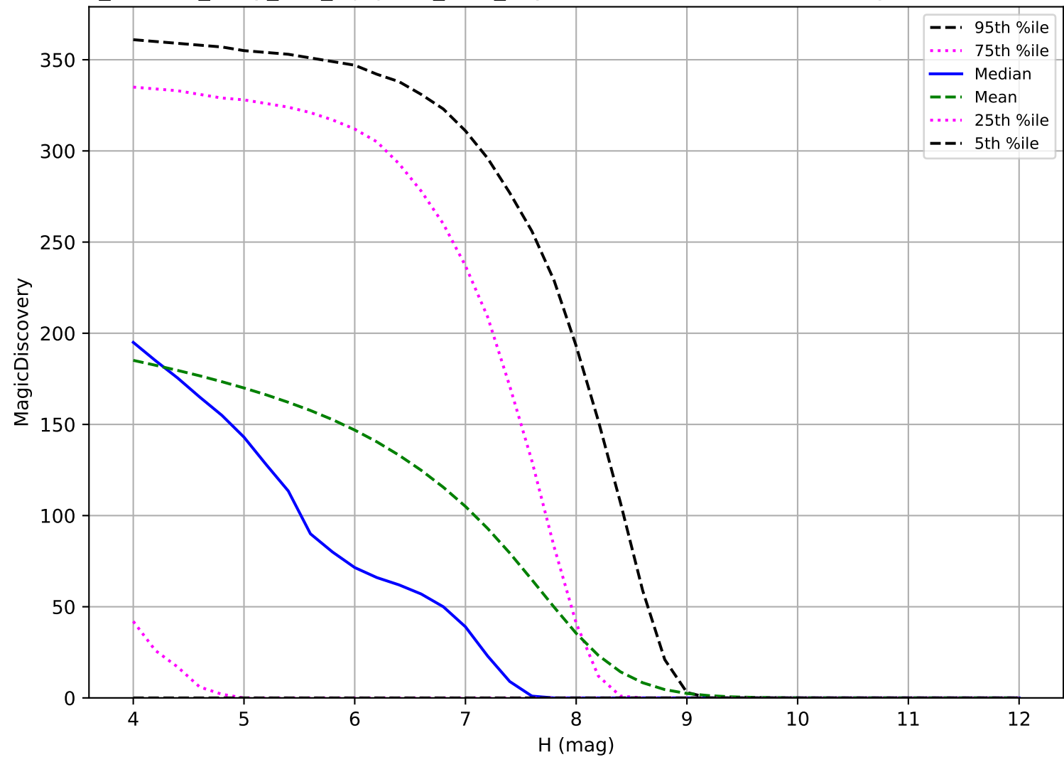
roll_uniform_early_half_mjdp180_v3.4_10yrs: TNO 6 detections in 60 nights detection loss
