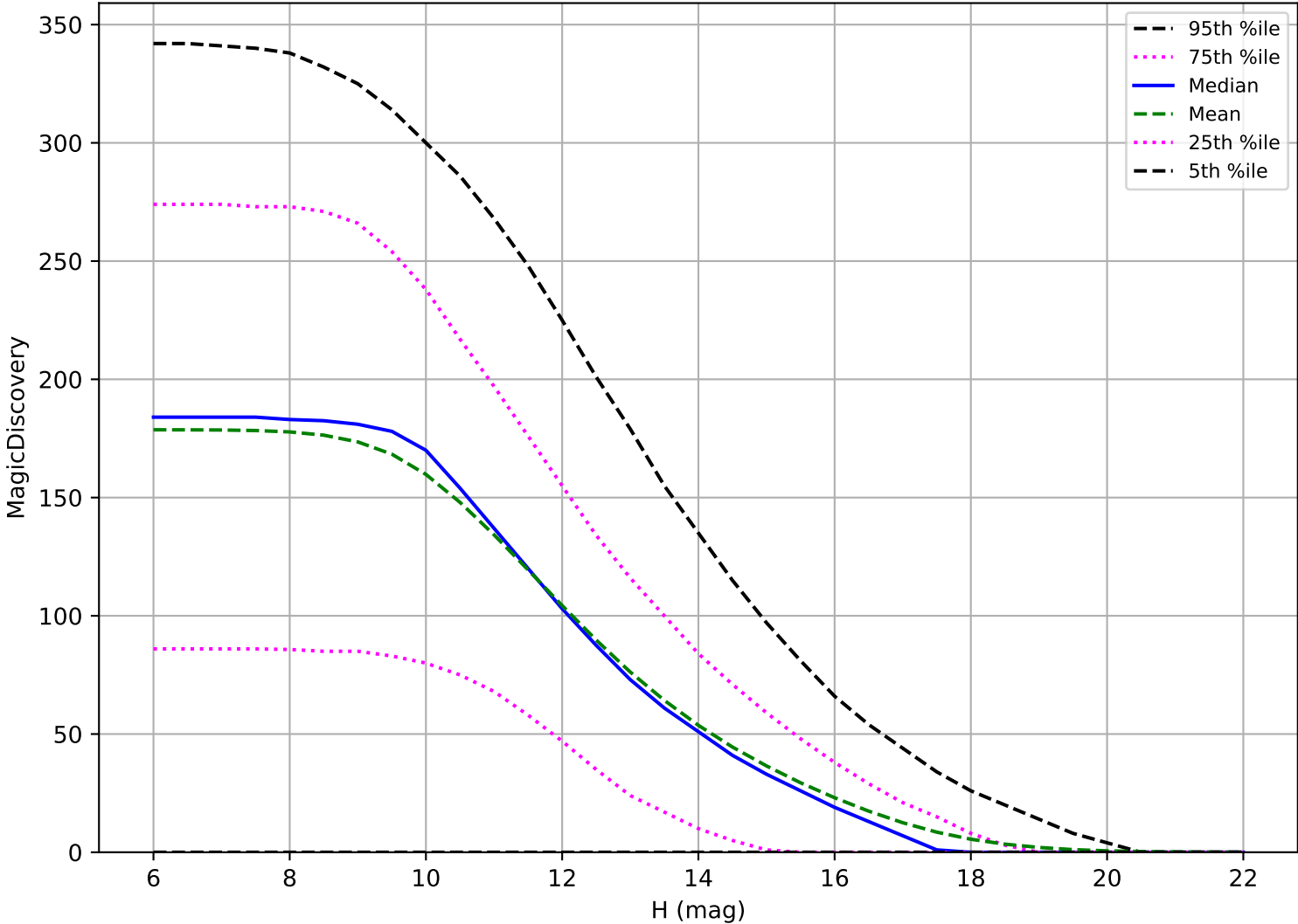
roll_uniform_early_half_mjdp180_v3.4_10yrs: OCC_r5 6 detections in 60 nights detection loss
