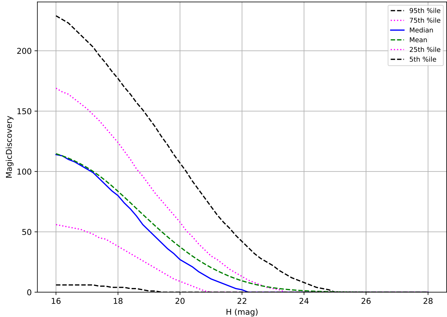
roll_uniform_early_half_mjdp180_v3.4_10yrs: NEO 6 detections in 60 nights detection loss
