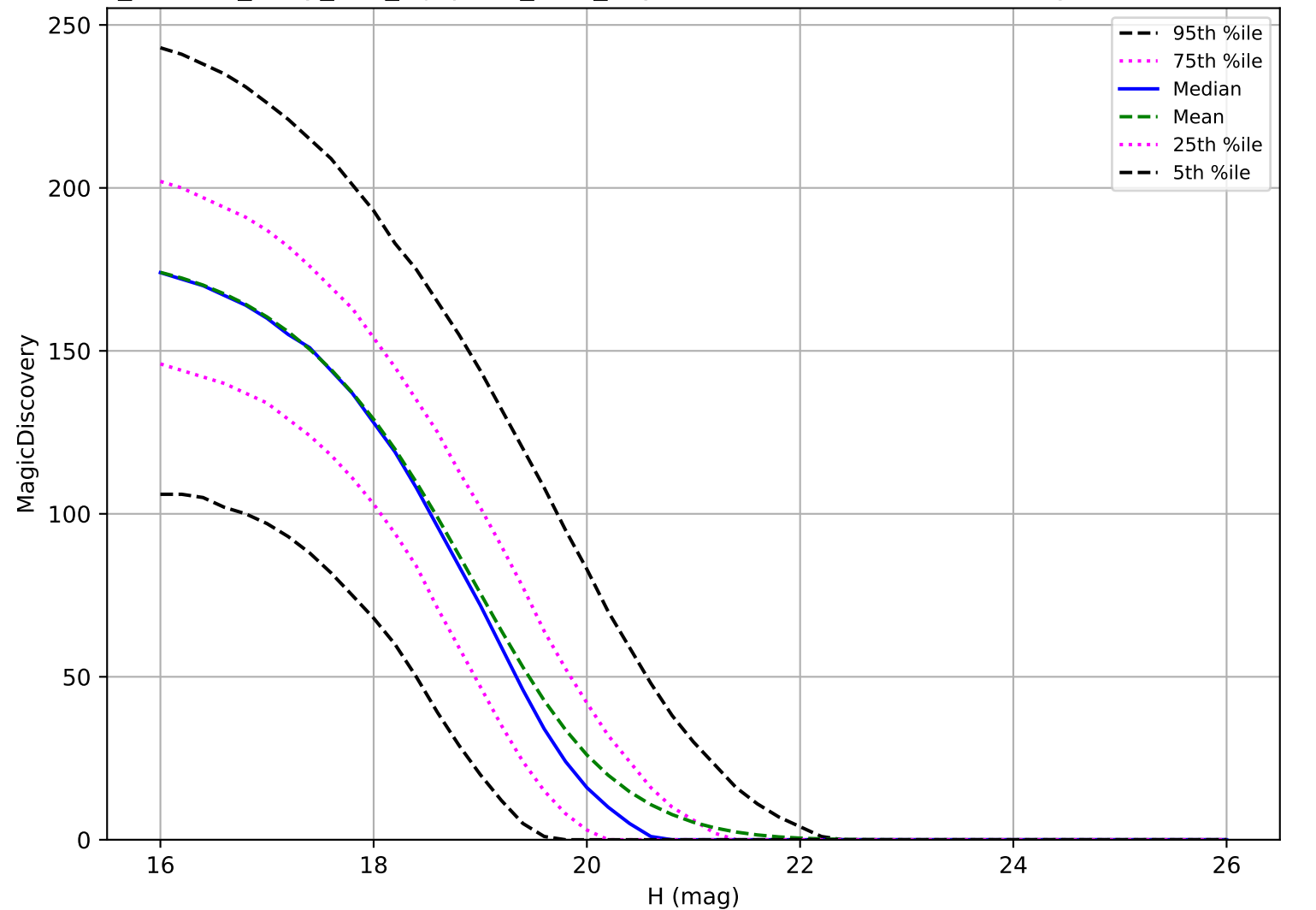
roll_uniform_early_half_mjdp180_v3.4_10yrs: MBA 6 detections in 60 nights detection loss
