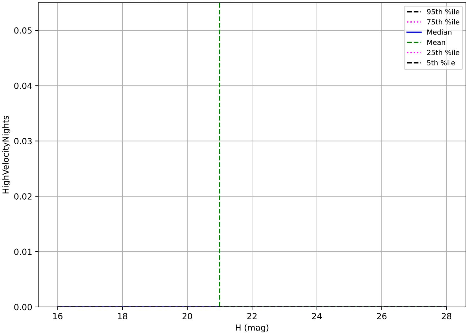
roll_uniform_early_half_mjdp180_v3.4_10yrs: Vatira High velocity pair detection loss
