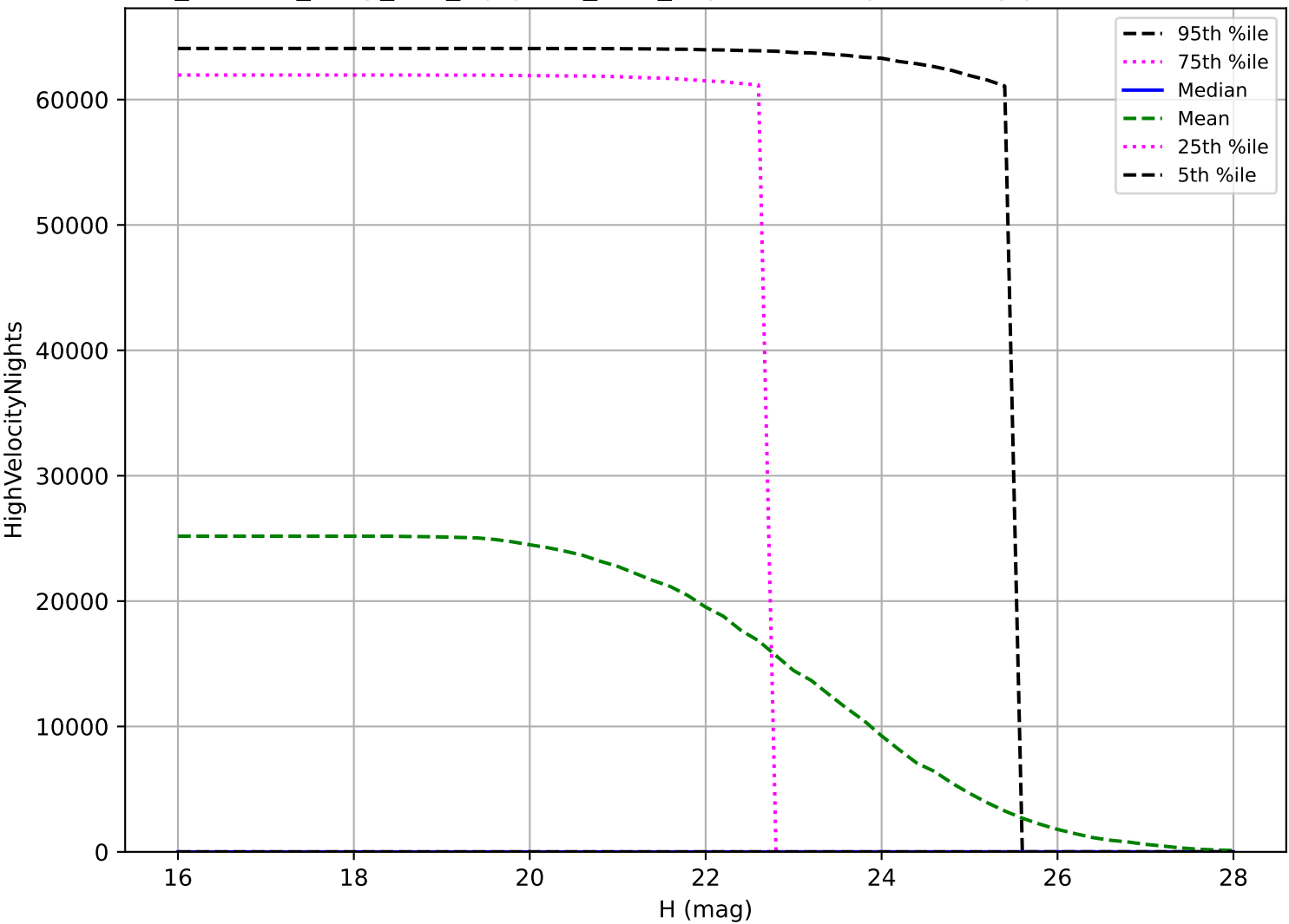
roll_uniform_early_half_mjdp180_v3.4_10yrs: PHA High velocity pair detection loss
