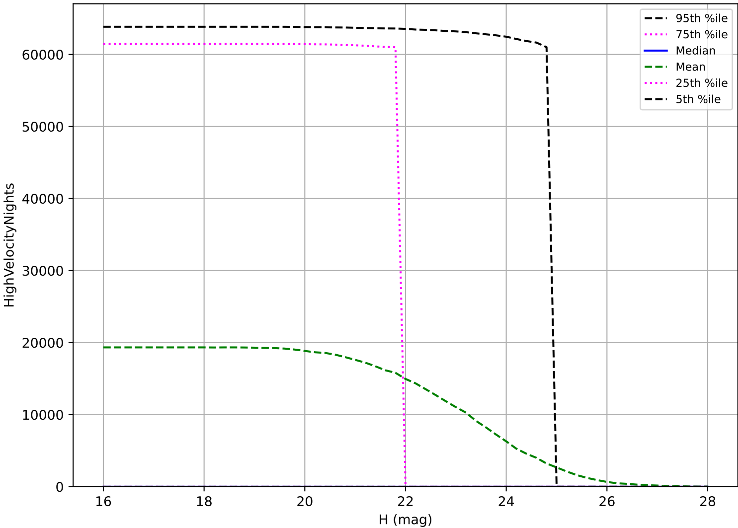
roll_uniform_early_half_mjdp180_v3.4_10yrs: NEO High velocity pair detection loss
