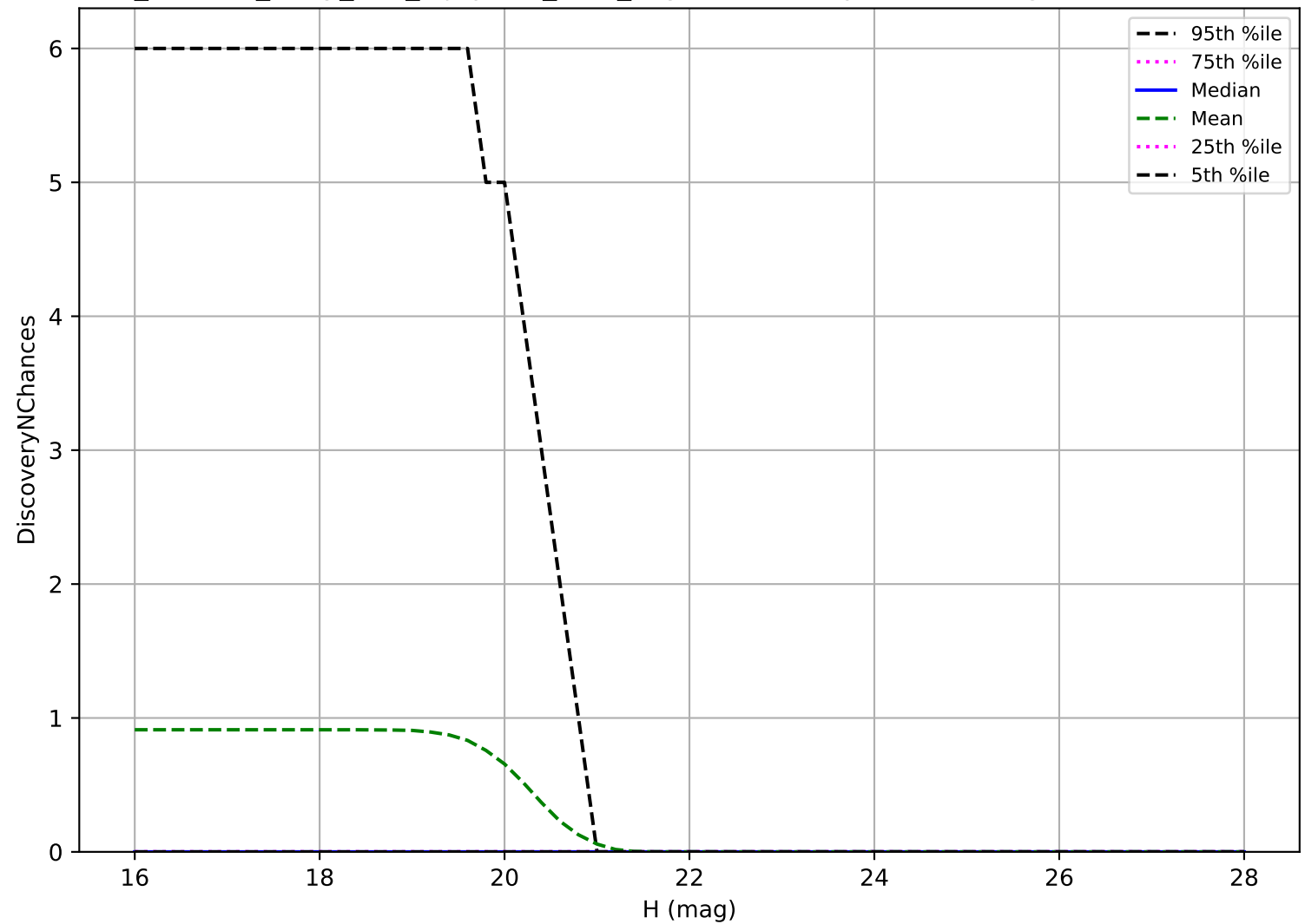
roll_uniform_early_half_mjdp180_v3.4_10yrs: Vatira 3 pairs in 15 nights detection loss
