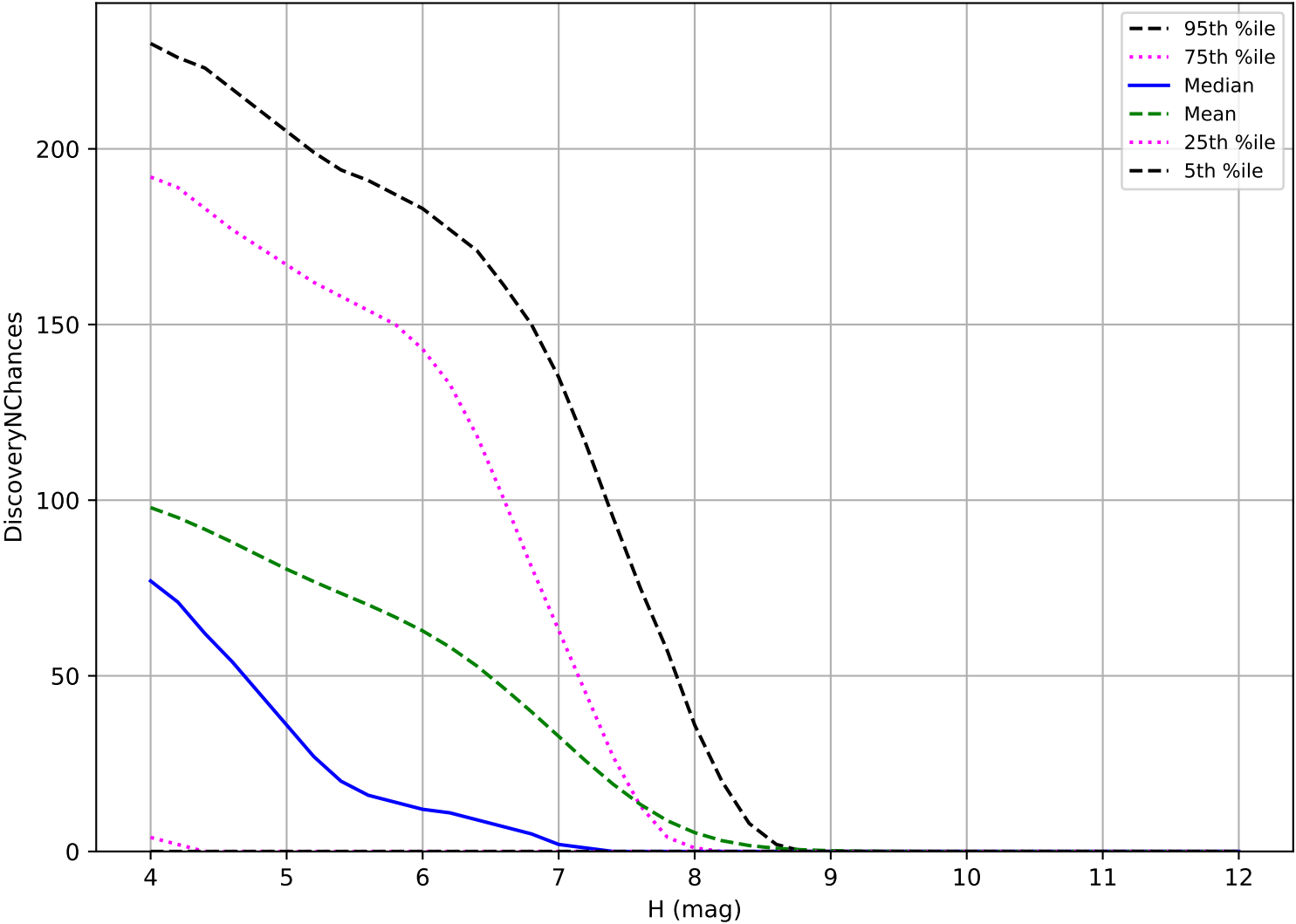
roll_uniform_early_half_mjdp180_v3.4_10yrs: TNO 3 pairs in 15 nights detection loss
