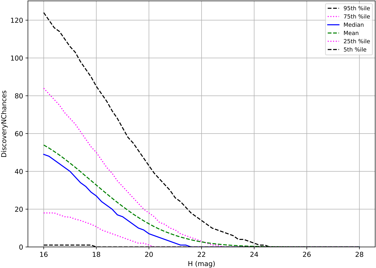
roll_uniform_early_half_mjdp180_v3.4_10yrs: PHA 3 pairs in 15 nights detection loss
