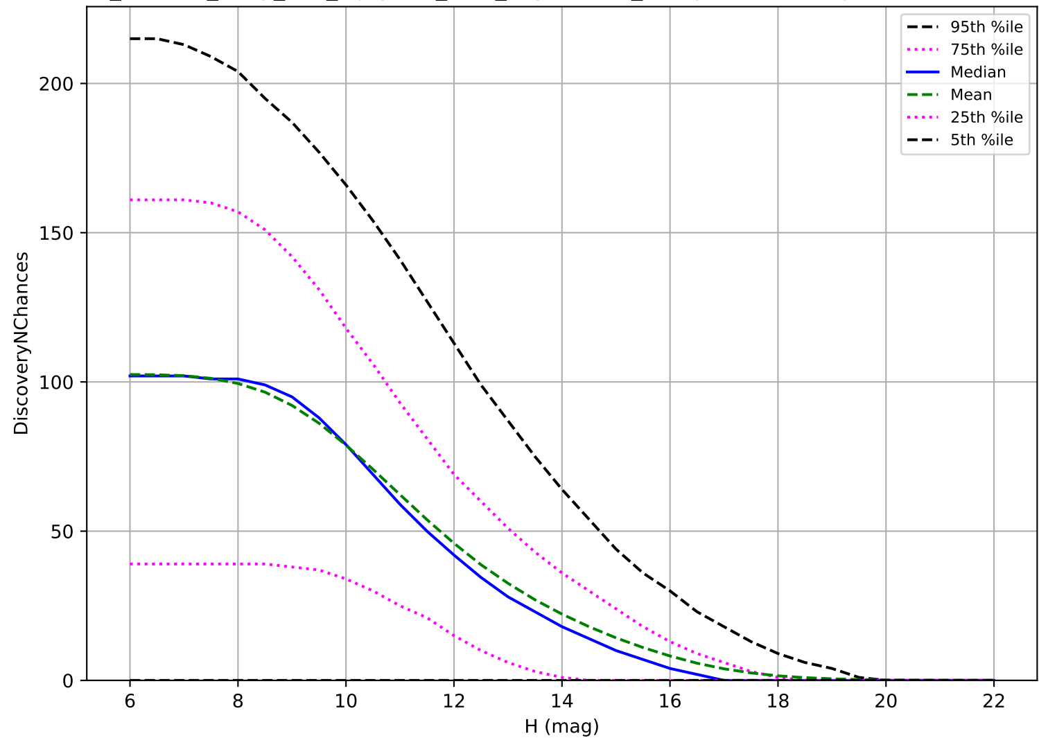
roll_uniform_early_half_mjdp180_v3.4_10yrs: OCC_r5 3 pairs in 15 nights detection loss
