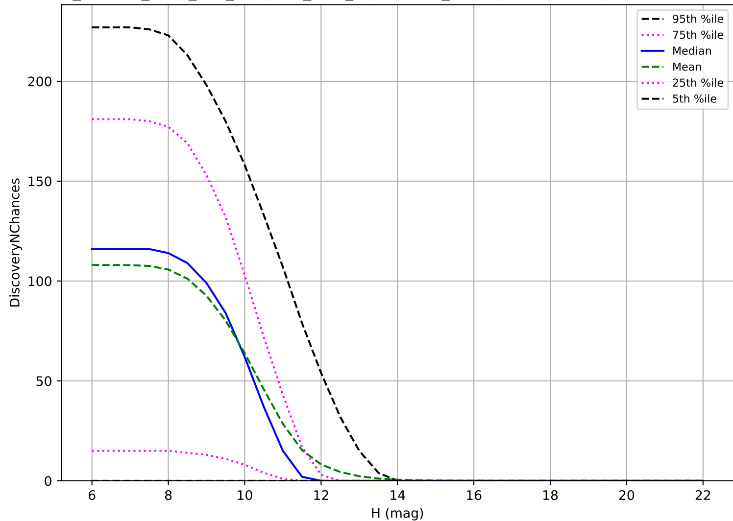
roll_uniform_early_half_mjdp180_v3.4_10yrs: OCC_r20 3 pairs in 15 nights detection loss
